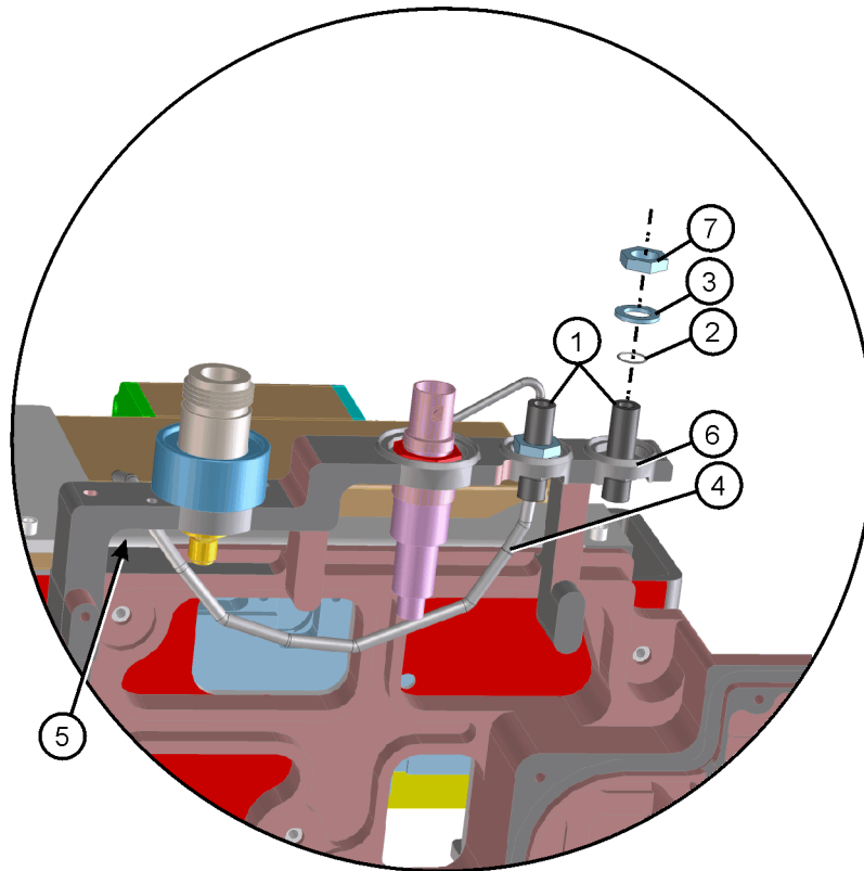
Figure 11 Installing SMA to SMA Connectors
